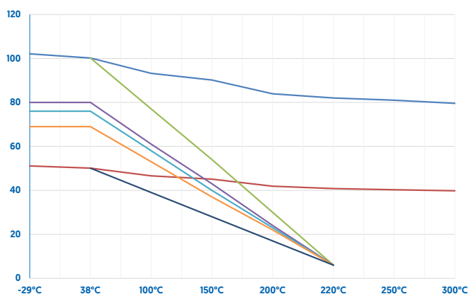
With TF 4103 seats
