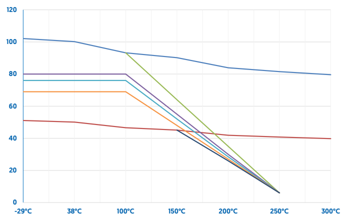
With PEEK seats
